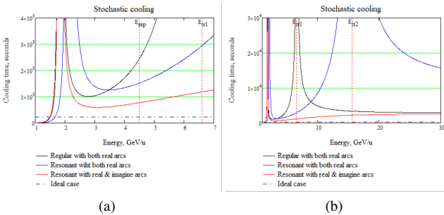
Fig. 5. (Color online) The dependence of stochastic cooling time on the energy for various lattices. Energy range (a) 1 – 7, (b) 0-30 GeV per nuclon.
