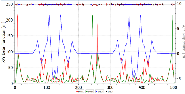
Fig. 2. (Color online) "Resonant" NICA magneto-optic adapted lattice with increased transition energy and missing magnet.
